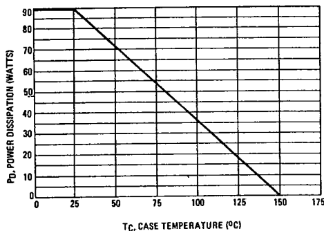
FIGURE 2 — POWER-TEMPERATURE DERATING CURVE
