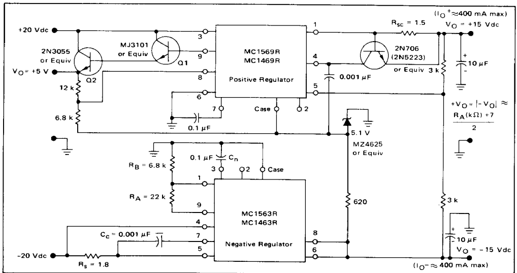
FIGURE 29 — A ±15 Vdc COMPLEMENTARY TRACKING REGULATOR WITH AUXILIARY +5.0 V SUPPLY
