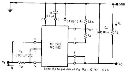
FIGURE 6 - LOAD REGULATION
