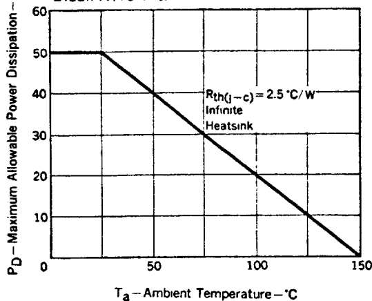
MAXIMUM ALLOWABLE POWER DISSIPATION vs. AMBIENT TEMPERATURE
