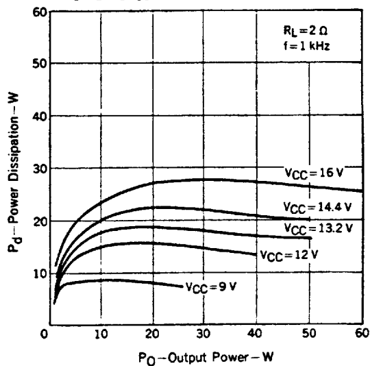
POWER DISSIPATION vs. OUTPUT POWER
