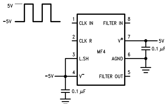
FIGURE 1. Schmitt Trigger R/C Oscillator
